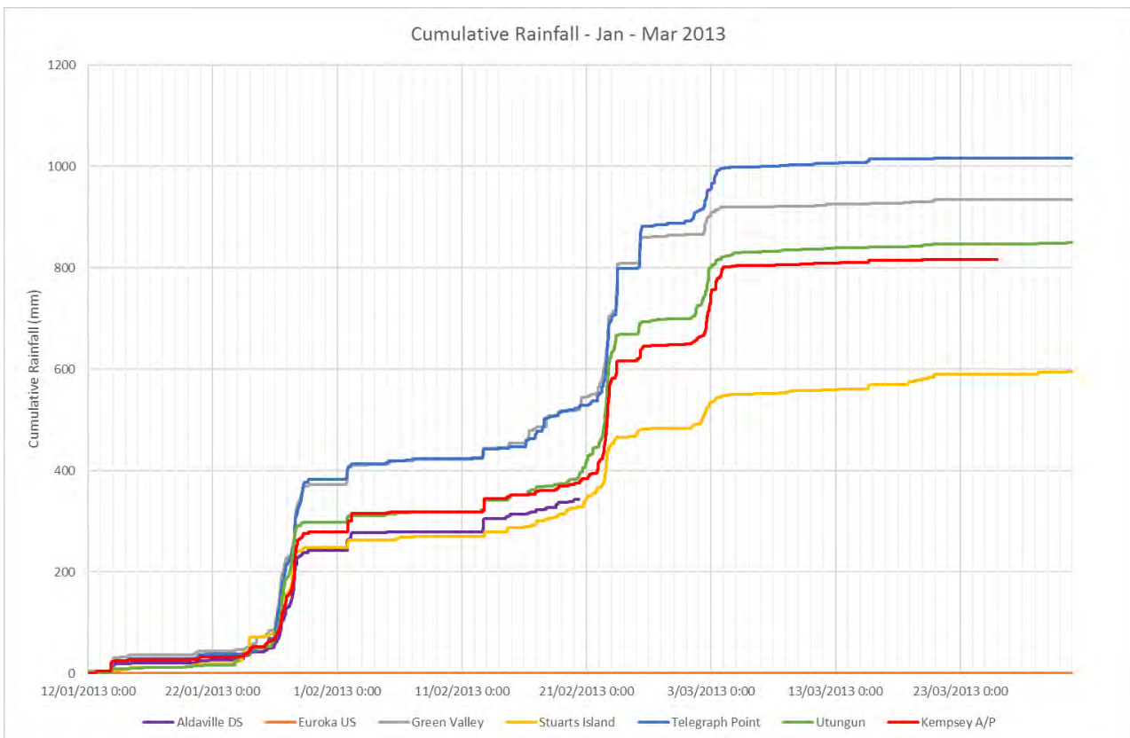
Figure A-2 Cumulative Rainfall for the Storm event of February 2013 and Preceding Period
